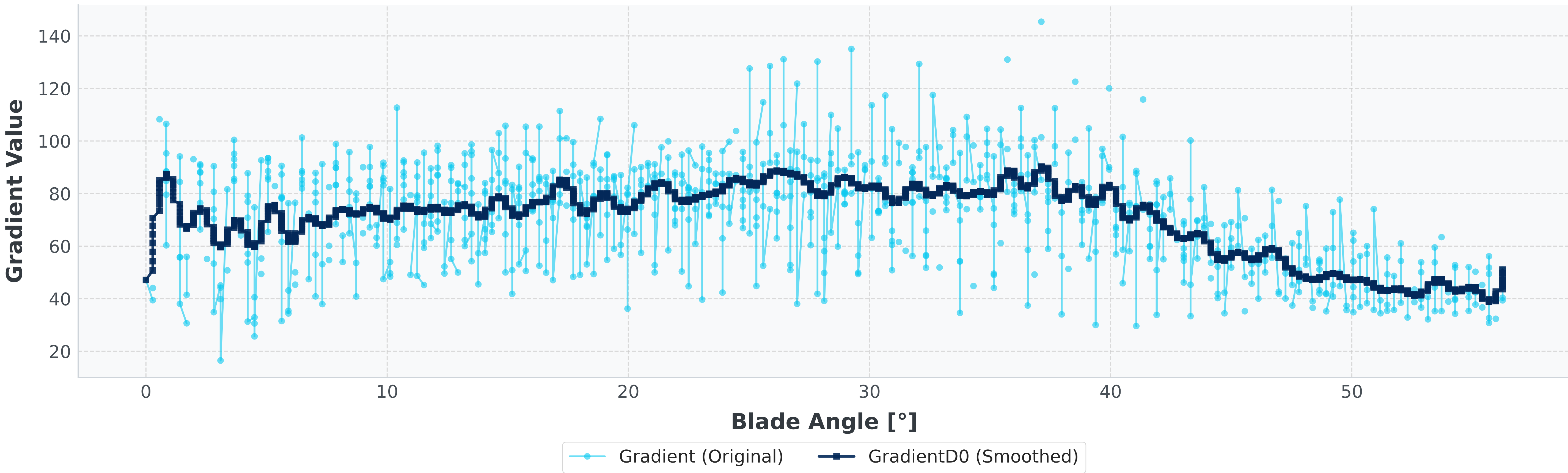
Cavity - Gradient (BLD Phase Averaged)
